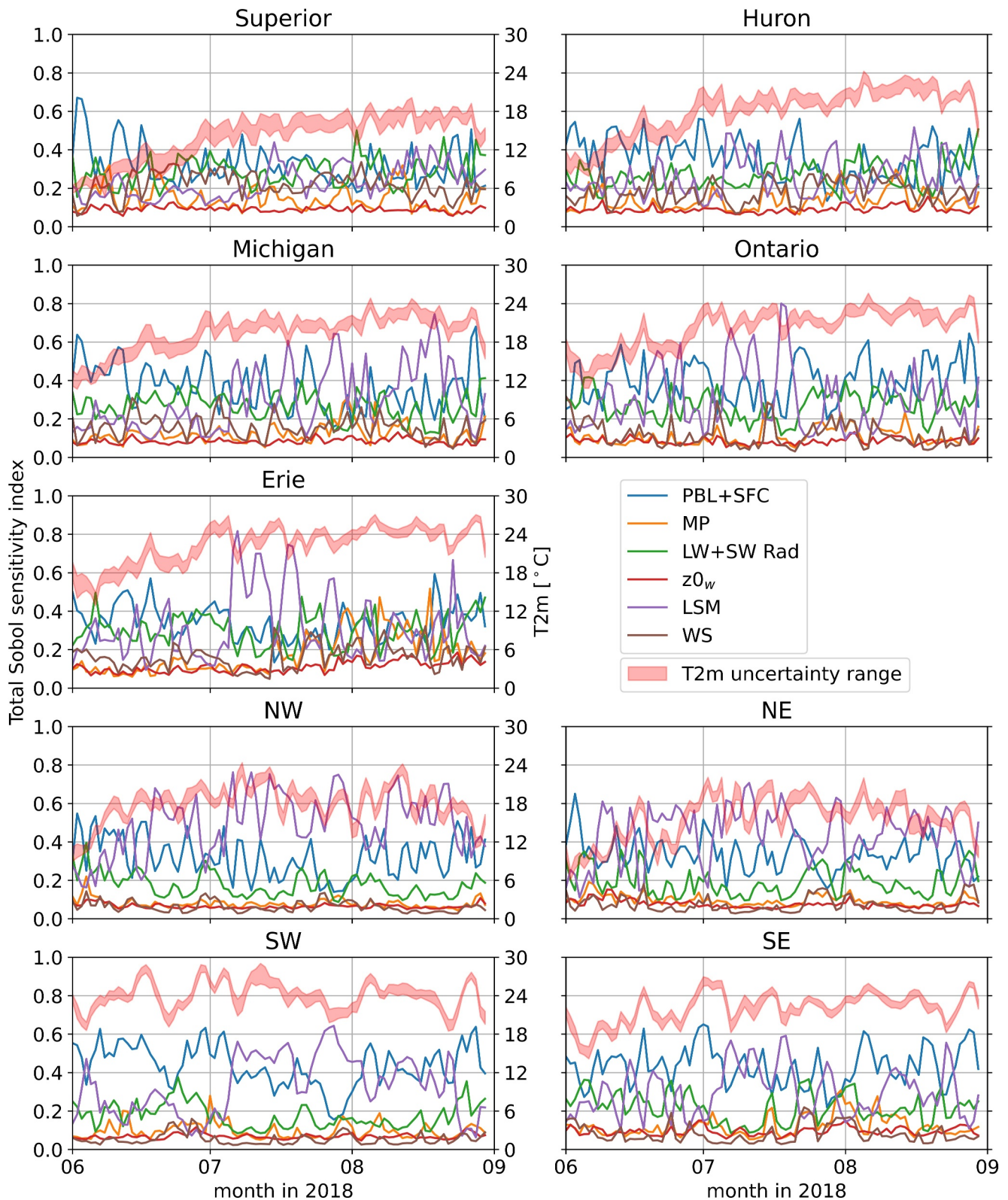
Figure 10. Temporal variation of T2m physics uncertainty (the range of the shaded area between the 5th and 95th percentiles) and total effect Sobol sensitivity indices for the six most important parameterizations (refer Figure 5) according to the spatially averaged surrogate model across each of the five Great Lakes and the four land quadrants (refer Figure 1).
